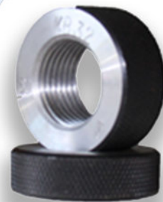
RING GAUGE GO RING GAUGE NO-GO RING GAUGE
